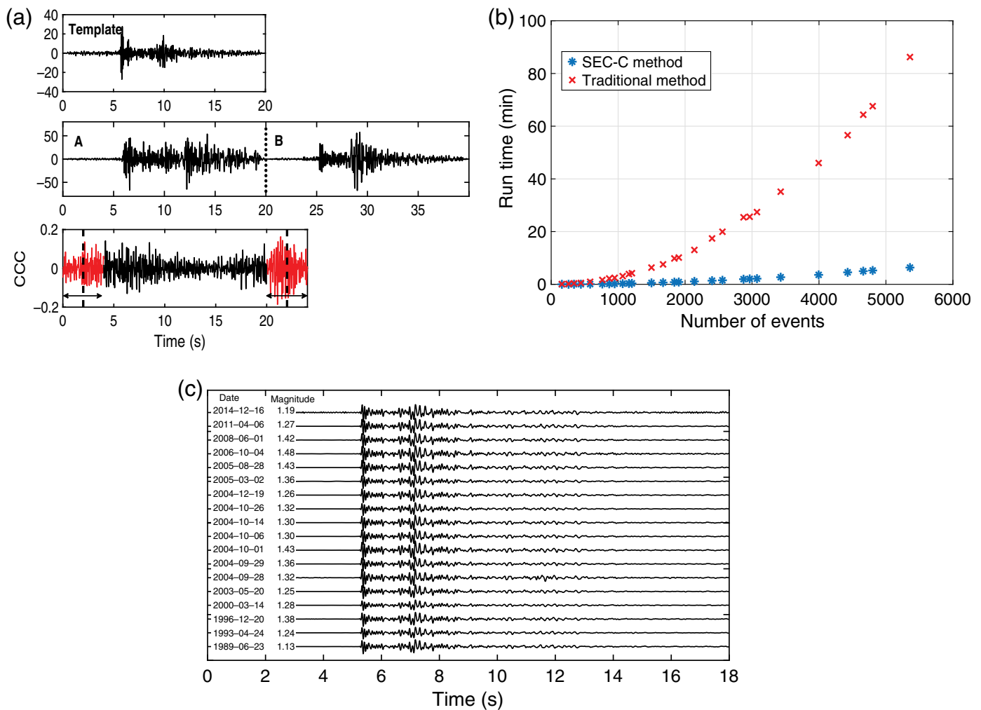
▲ Figure 4. (a) An example shows how we use the SEC-C method to calculate CCCs for individual event waveforms. From top to bottom: a template, concatenated waveforms A and B, and CCC between the template and the concatenated waveform. Portions of the CCC function indicated by double-headed arrows are the scientifically useful calculated CCCs and the remainder the unnecessary CCCs calculated in this process. Dashed lines indicate the CCC when the template is aligned with A and B based on P -arrival phase information. The majority of CCC calculations are unnecessary (more than 83%). (b) Computational time comparison between SEC-C method and the traditional method of searching for REs in different data sets containing different numbers of events. Both of these methods show computation time proportional to the square of the number of events, n (i.e., O(n^2) ). This comparison shows that the SEC-C method is 10.8–15.5 times faster for data sets ranging from hundreds to thousands of events and has a mean improvement of 12.1 times faster in general. (c) One example of a RE family detected by the SEC-C method using waveform data from seismic station PGH (see Fig. 3a for locations of the RE family and PGH). The color version of this figure is available only in the electronic edition.
